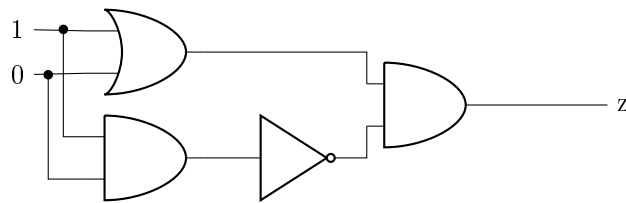
Figure 1: Logic circuit 1
